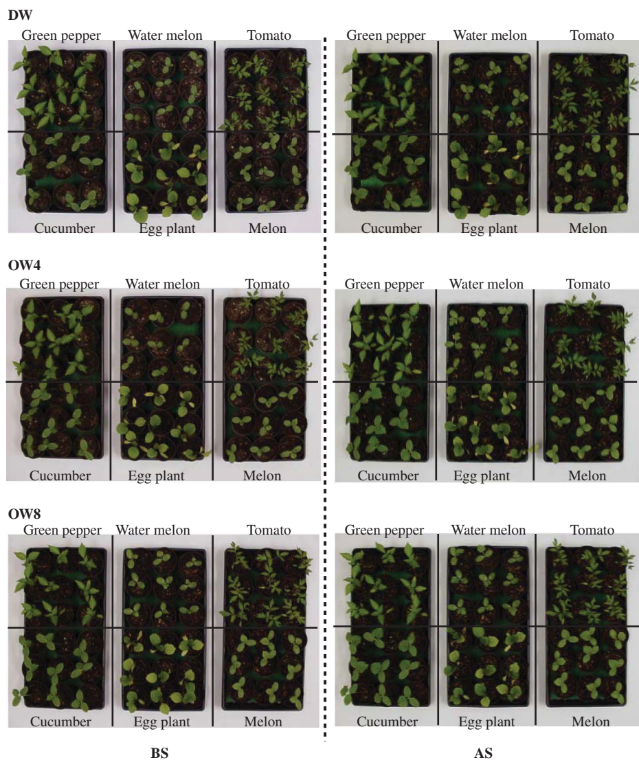
FIGURE 1. Seedlings of green pepper, watermelon, tomato, cucumber, eggplant, and melon before and after spraying (BS and AS) distilled water (DW) or ozonated water (OW) with a dissolved ozone concentration (DOC) of 4.0 \text{ mg L}^{-1} (OW4) or 8.0 \text{ mg L}^{-1} (OW8). In all cases, the water was sprayed twice everyday (10 a.m. and 2 p.m.) on 3 successive days (sprayed a total of 6 times in 3 d).
